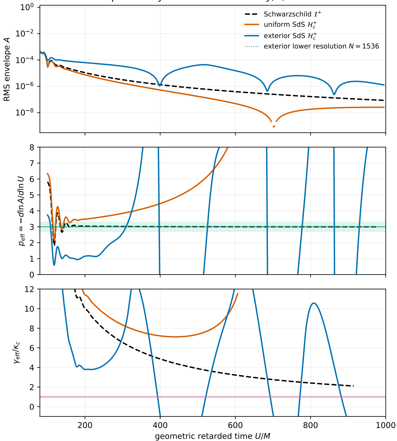
Dipole decay at the outer boundary, L/M = 640
