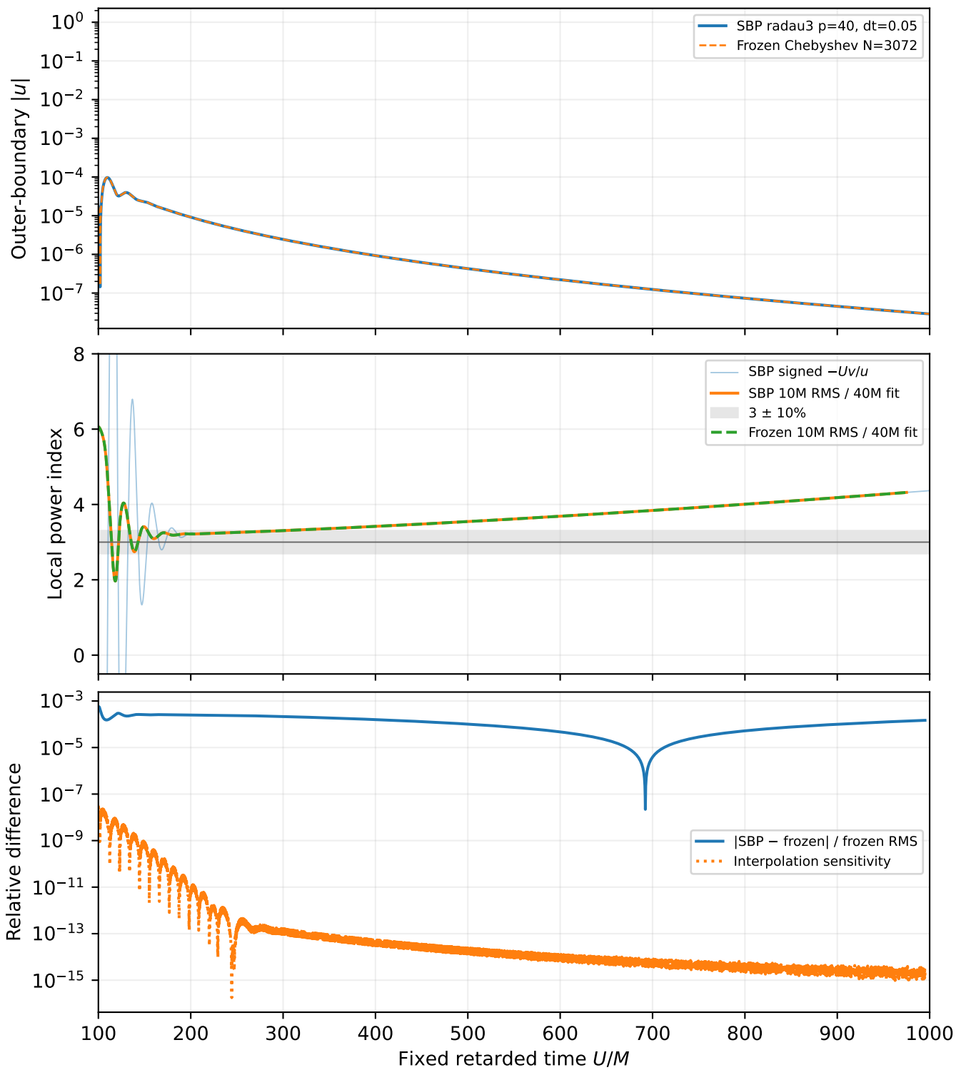
uniform L640 xi1o6 ell1 radau3 Pilot comparison: diagnostic, not a production replacement
