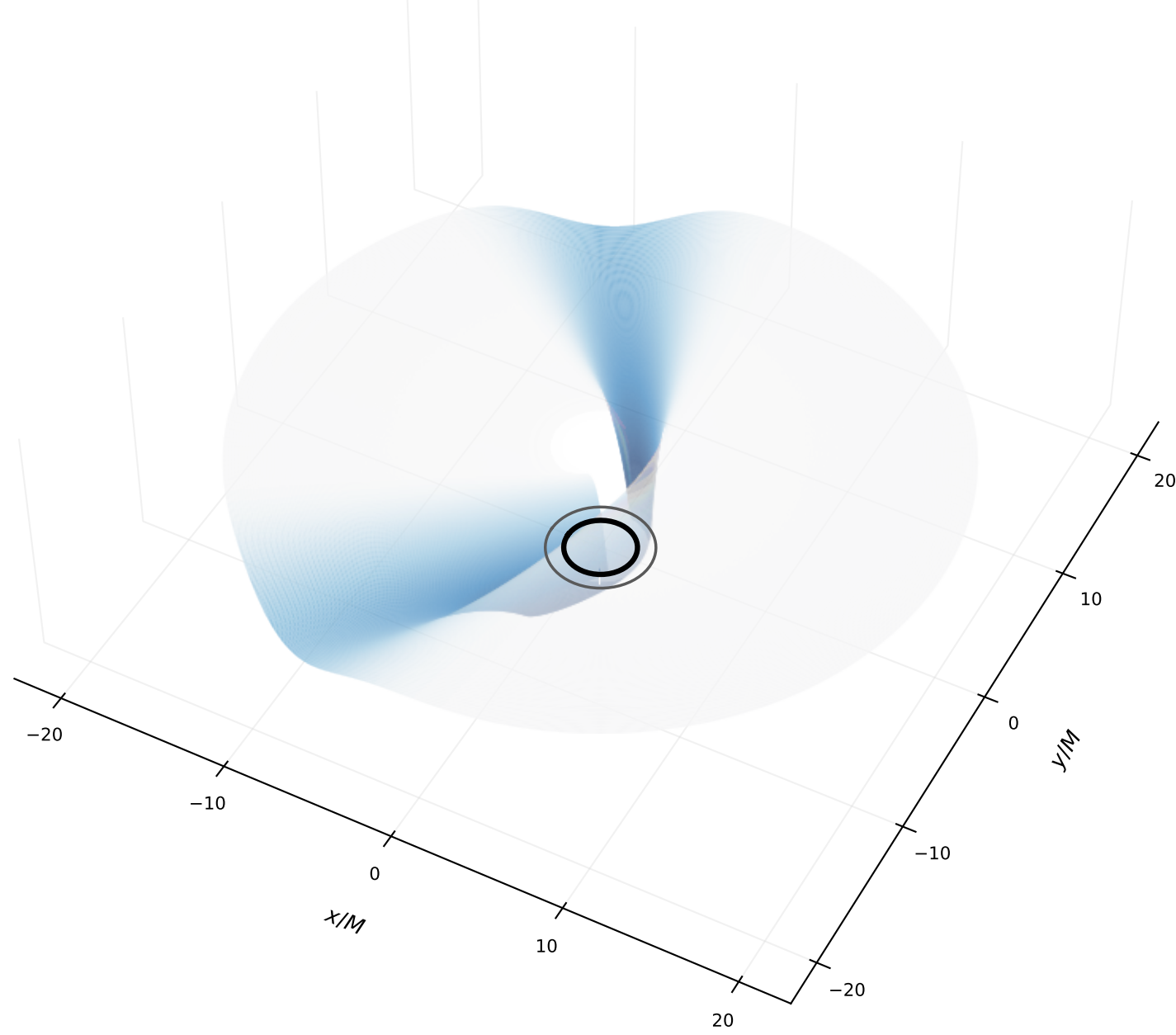
Wavefront as height and colour, \tau/M = 40.00 , clipped at \pm 3.4e - 03 , the 60th percentile of the disturbed region
