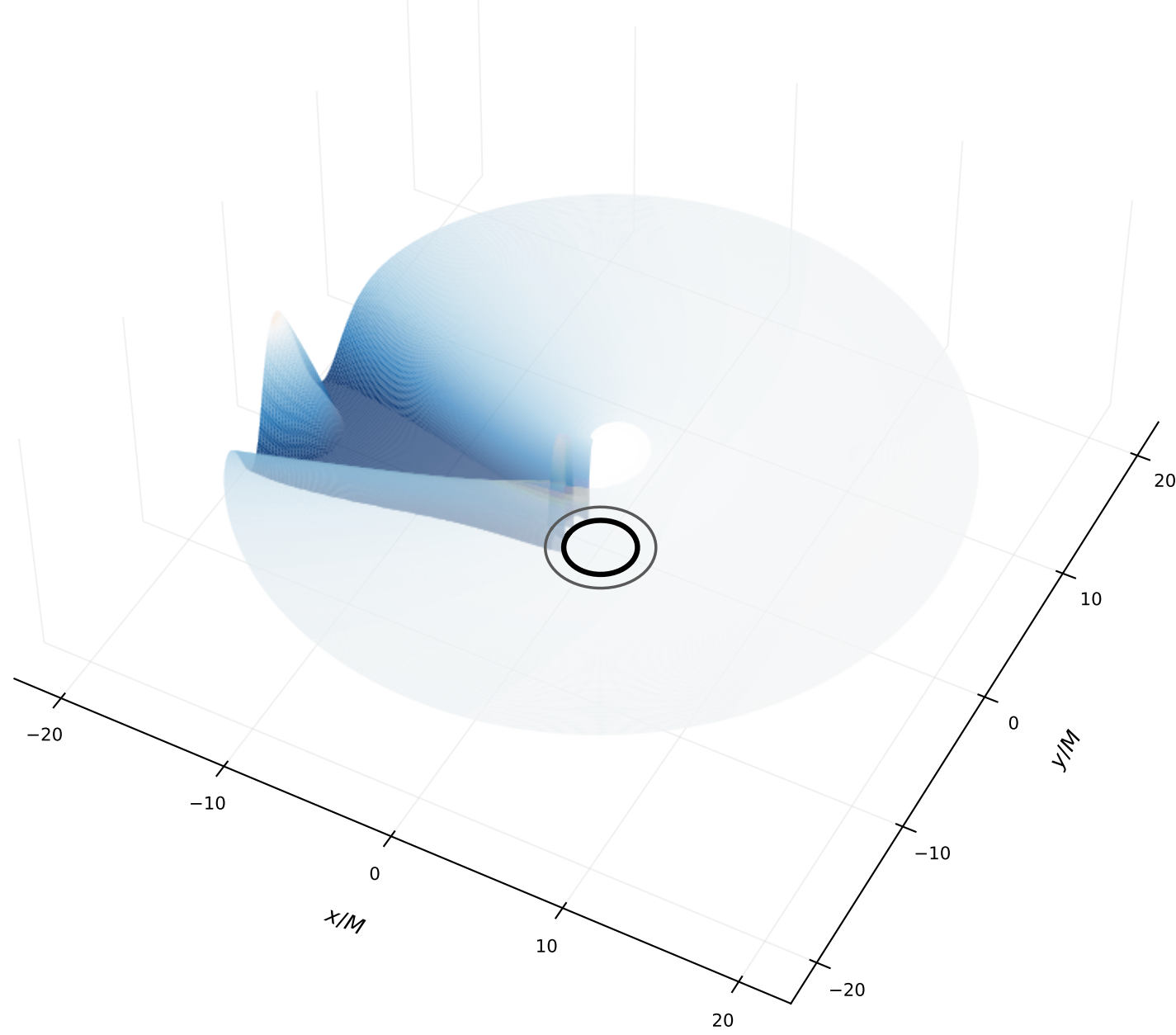
Wavefront as height and colour, \tau/M = 48.00 , clipped at \pm 1.7e - 03 , the 60th percentile of the disturbed region
