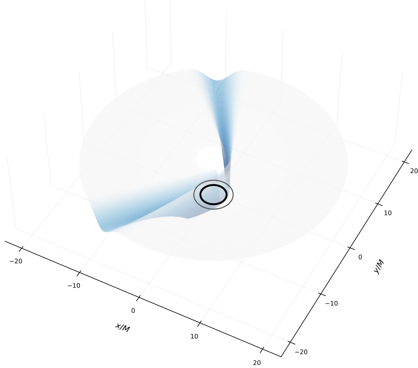
Wavefront as height and colour, \tau/M = 40.00 , clipped at \pm 6.7e - 03 , the 60th percentile of the disturbed region
