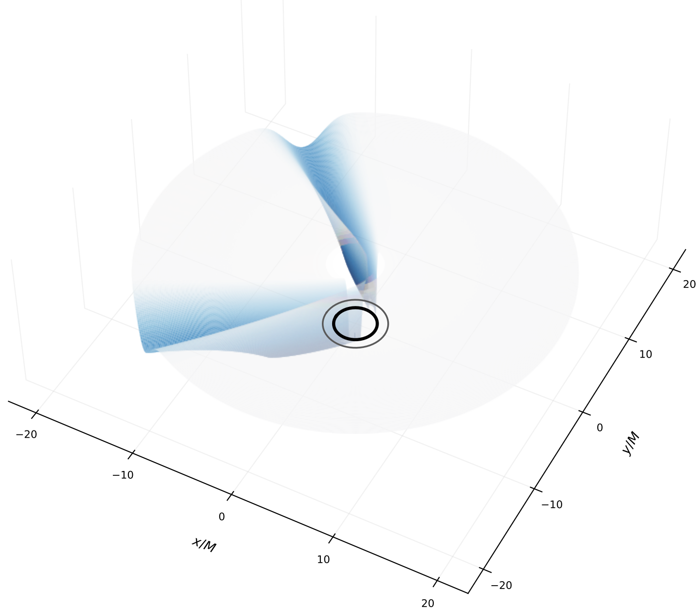
Wavefront as height and colour, \tau/M = 42.00 , clipped at \pm 4.8e - 03 , the 60th percentile of the disturbed region
