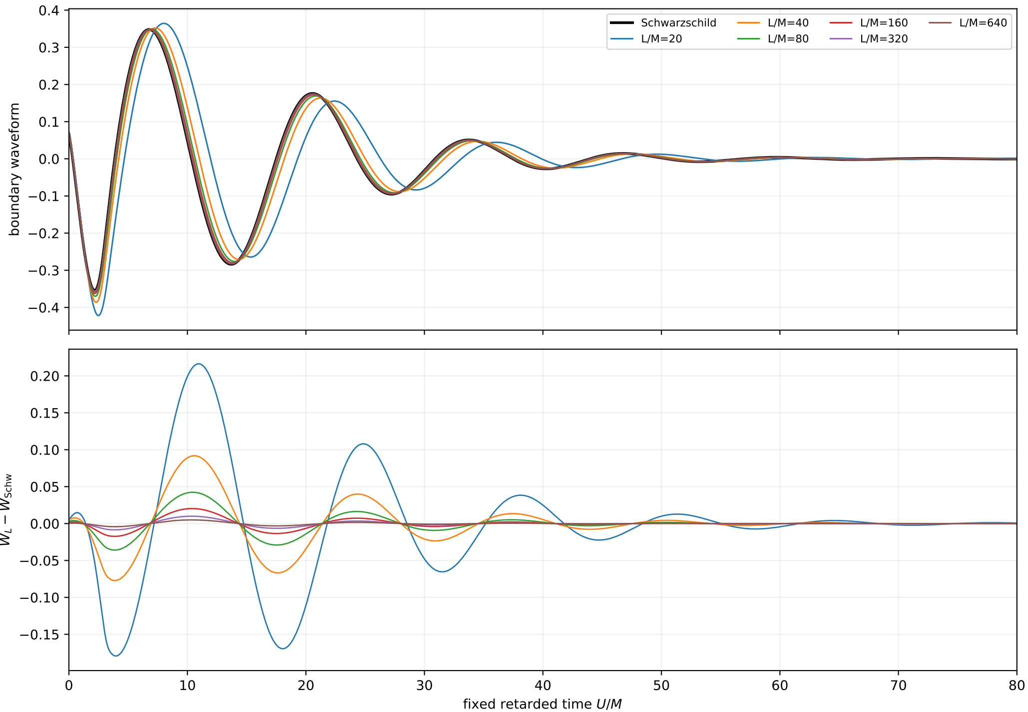
Pure \ell = 2 fixed-data regulator sequence
