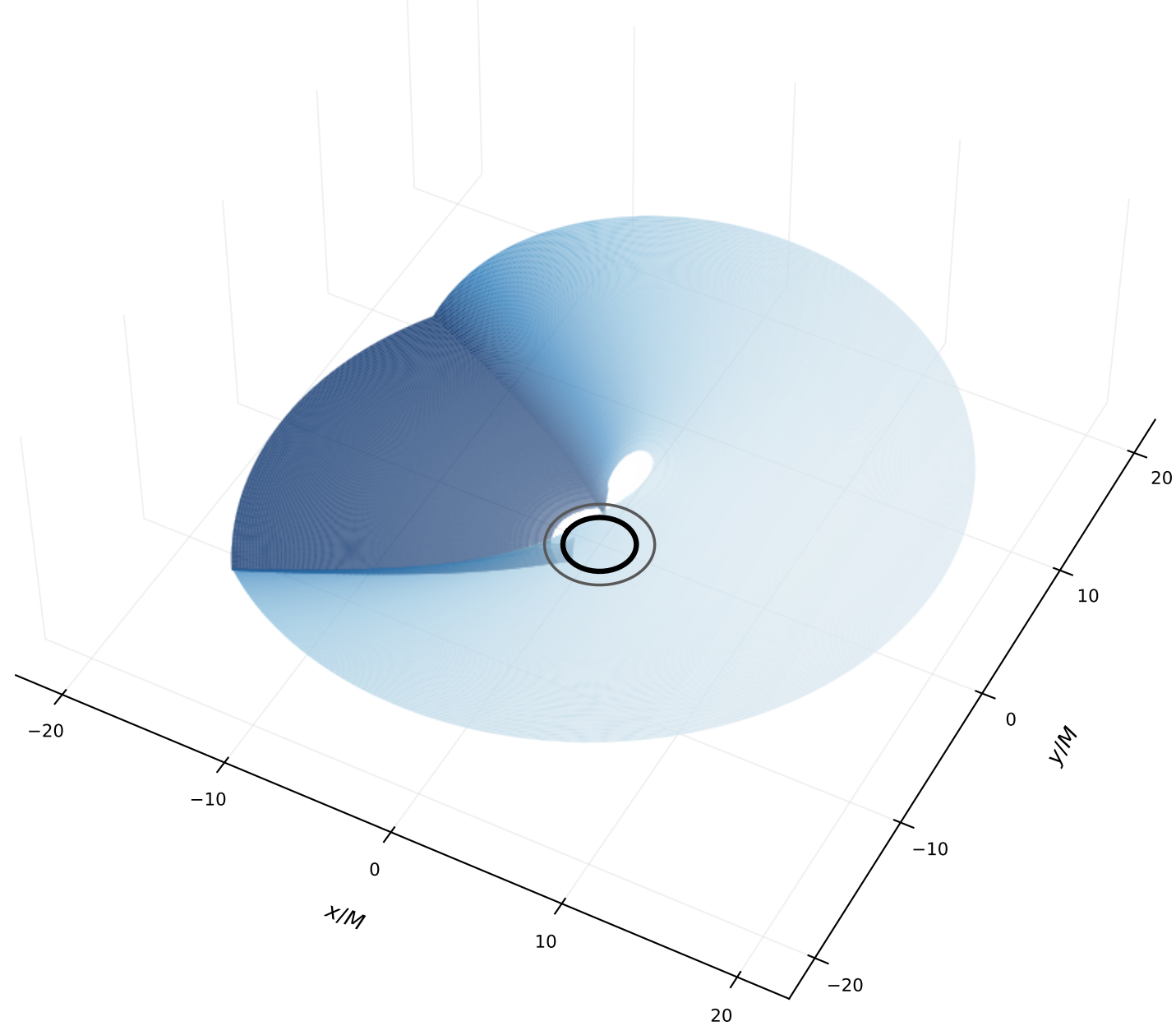
Wavefront as height and colour, \tau/M = 47.75 , clipped at \pm 2.5e - 04
