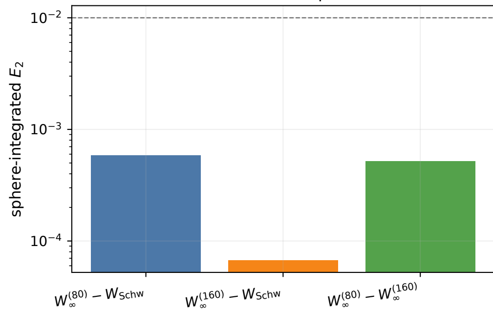
(b) Nested extrapolants
