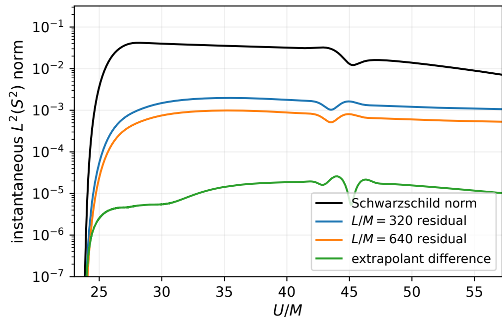
(c) Modal residuals
