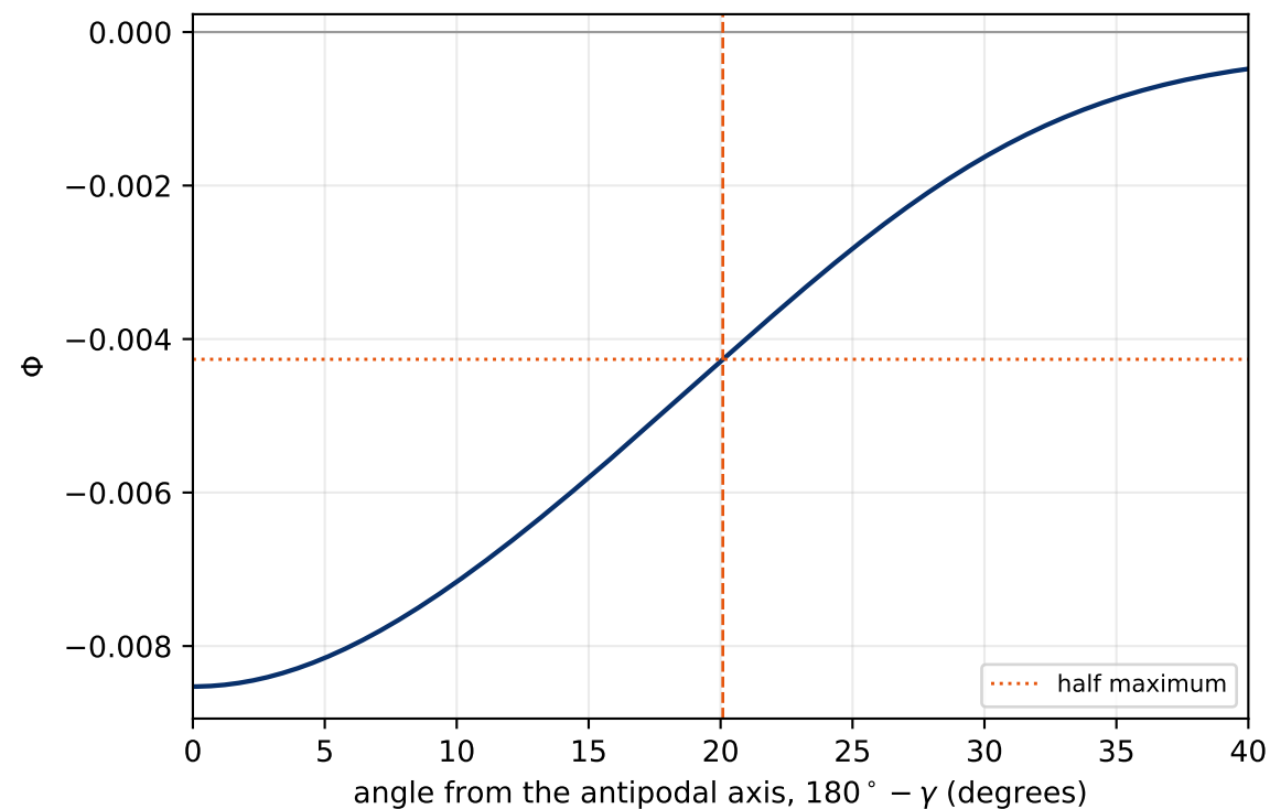
Angular-truncation convergence of the focus
