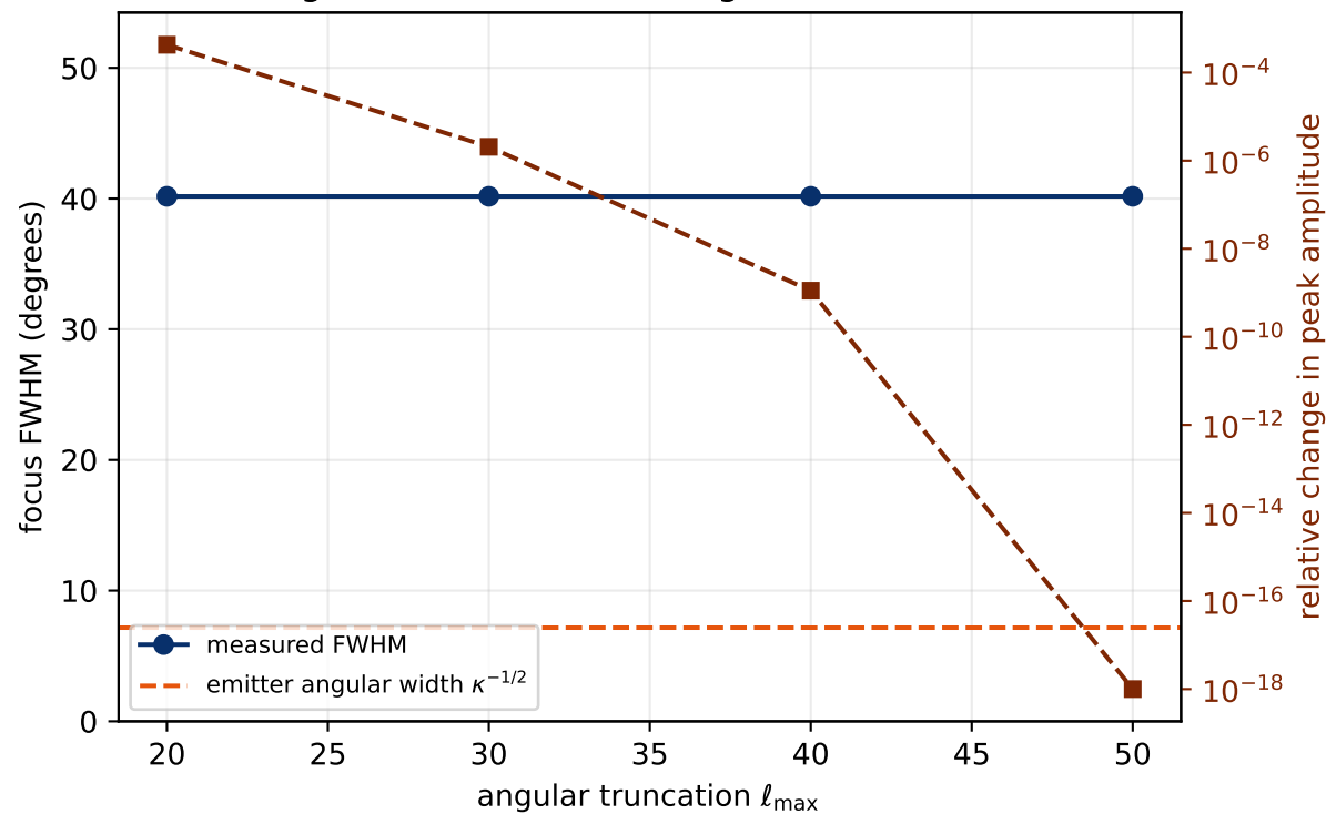
Angular-truncation convergence of the focus
