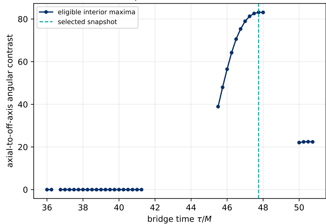
Snapshot-selection metric
