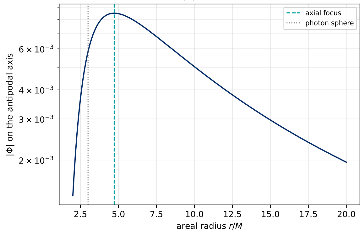
Snapshot-selection metric
