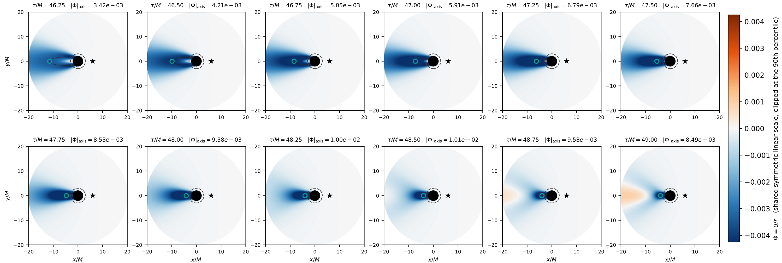
Equatorial section through the antipodal caustic, emitter at r = 6M , L/M = 80
