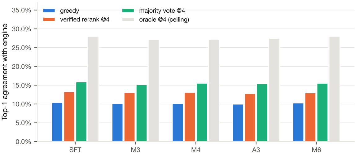
Selecting among 4 sampled traces
