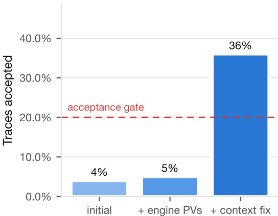
(a) Acceptance rate
