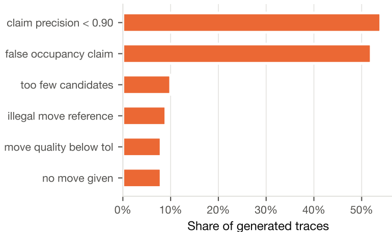
(b) Why traces are rejected
