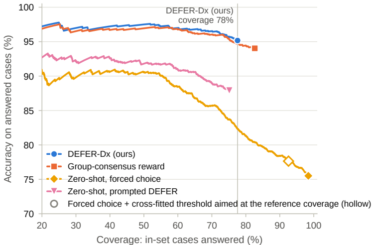
a Risk-coverage on CDM val + test (480 cases, 3 seeds)
