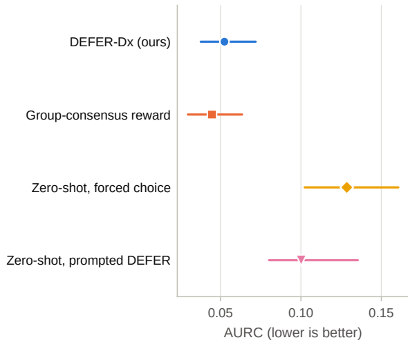
b Area under the risk-coverage curve ↓
