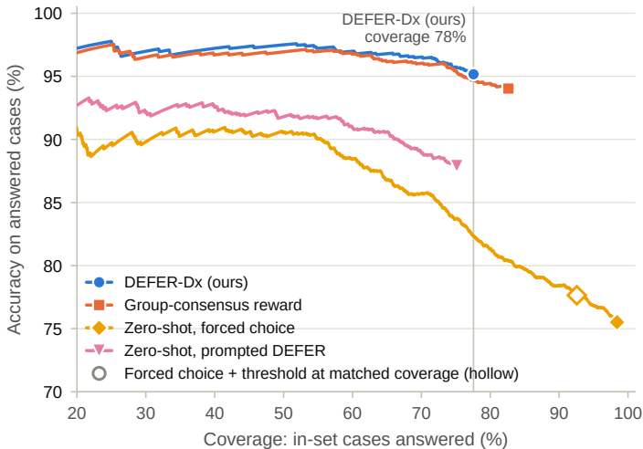
a Risk-coverage on CDM val + test (480 cases, 3 seeds)
