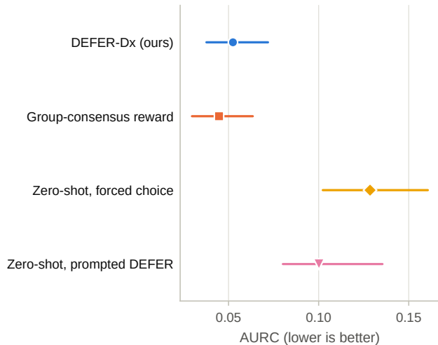
b Area under the risk-coverage curve ↓
