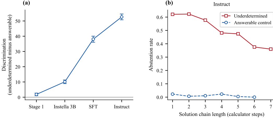
Figure 1: Left: discrimination between underdetermined and answerable problems across the training pipeline. Right: abstention against solution chain length at the instruct checkpoint, with the answerable control on the same axes. The control is flat, so the decay is specific to detecting that premises are missing.
