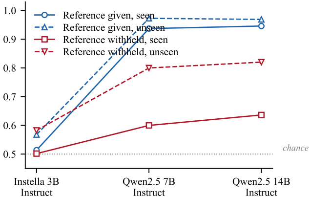
Balanced accuracy
