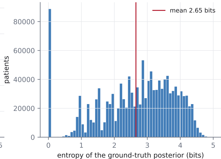
Targets are genuinely distributional, not one-hot
