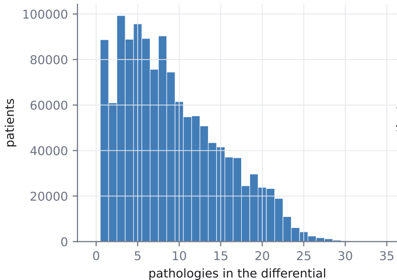
Differential support (median 8 of 49)
