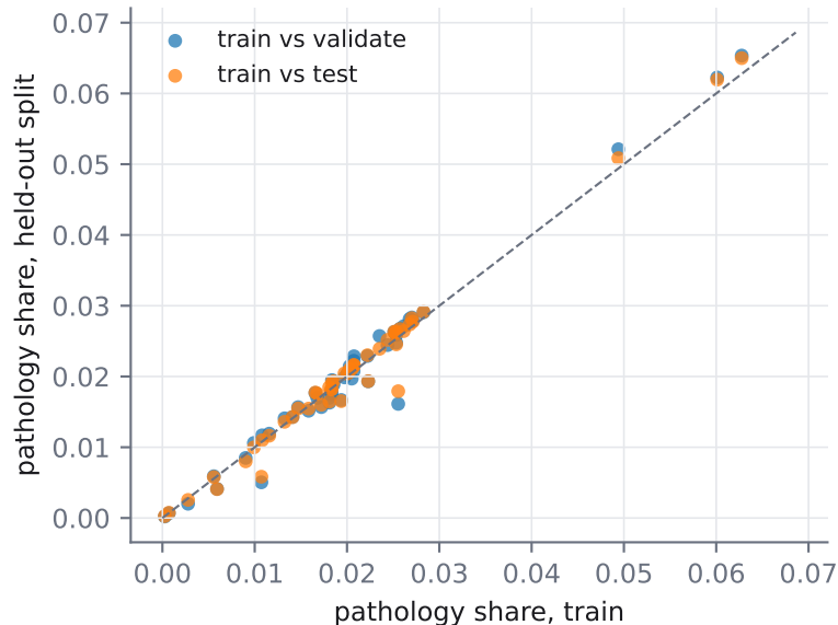
Splits are distributionally matched (PSI &lt; 0.013)
