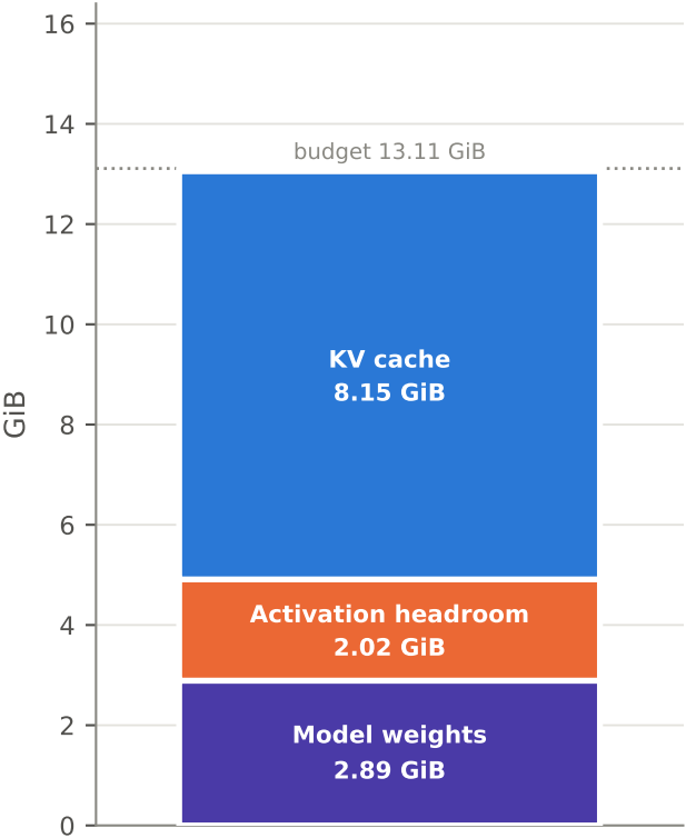
What vLLM reserves at startup
