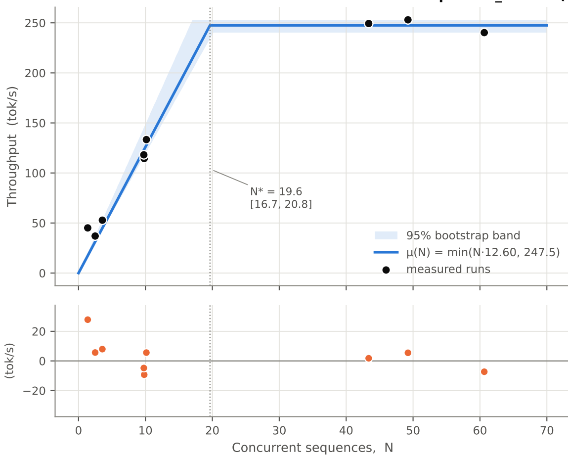
Fitted service law vs measurement — workload phase1_mixed ( R^2 = 0.983 , MAPE = 12.7%)
