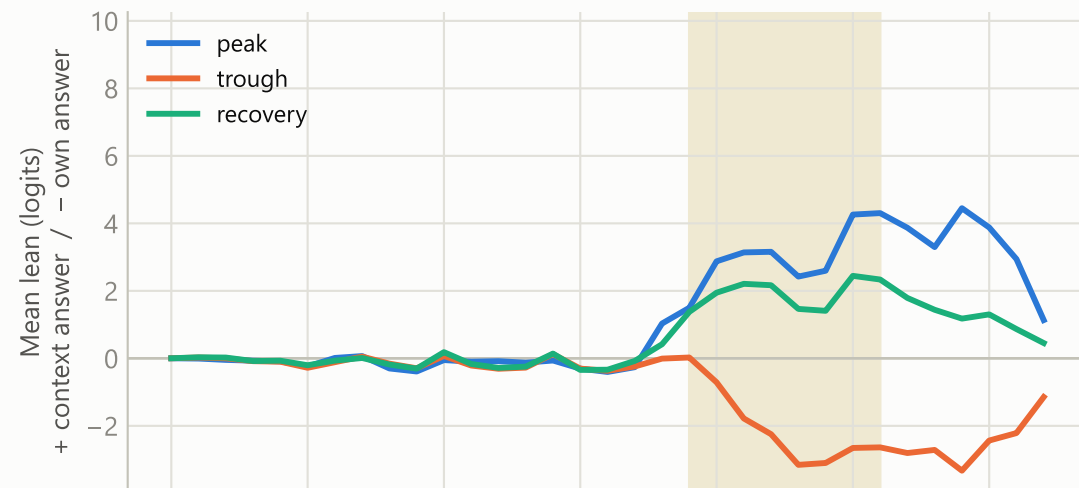
Alpaca — flipping capitals (n = 36)
