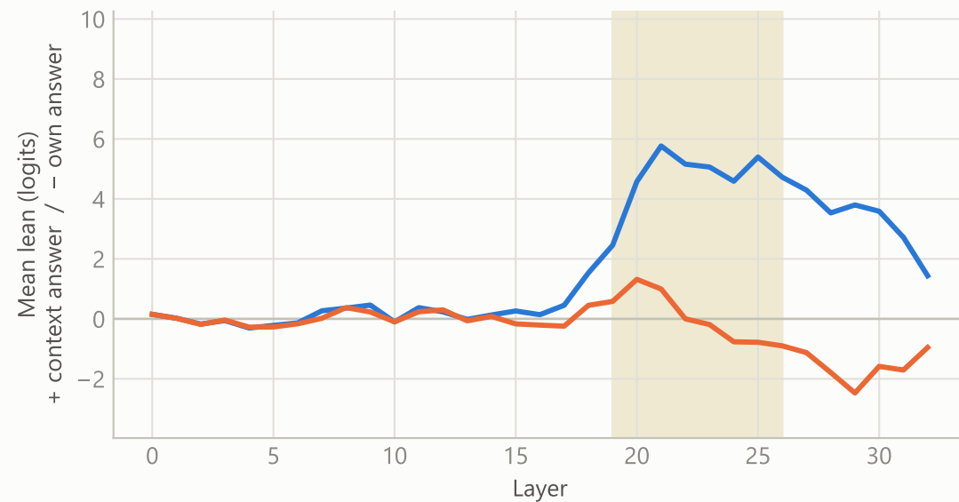
Alpaca — flipping capitals (n = 36)
