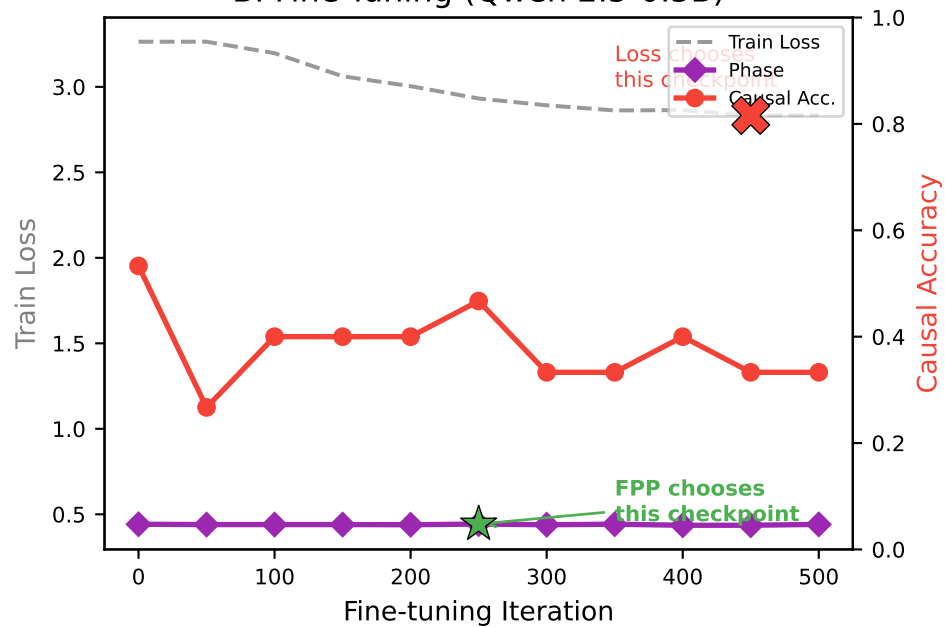
B. Fine-Tuning (Qwen 2.5-0.5B)
