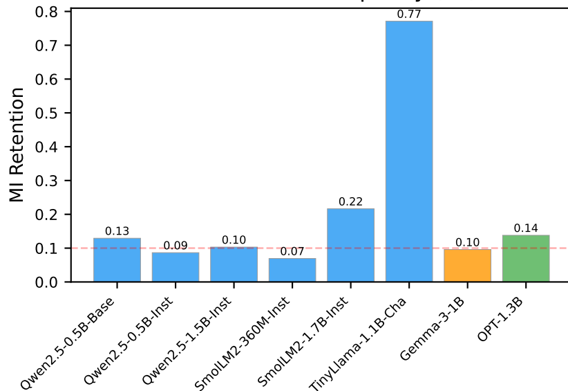
D. GS vs MI: Orthogonal Dimensions
