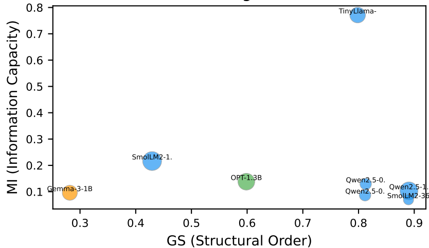
D. GS vs MI: Orthogonal Dimensions
