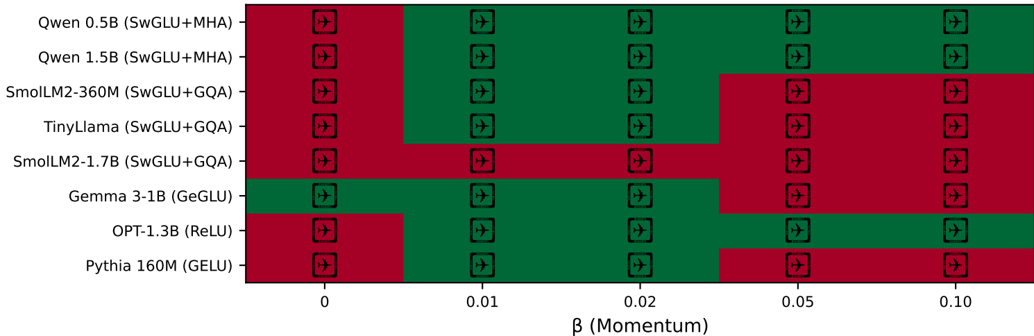
Figure 3: Safe \beta Injection Range by Architecture Family
