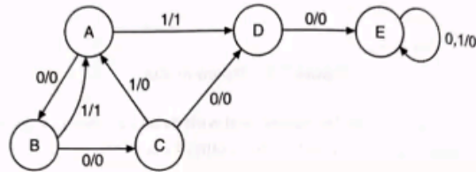
Figure 7.9 State diagram.
