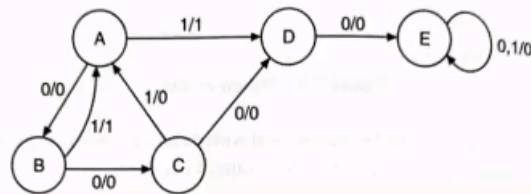
Figure 7.9 State diagram.
