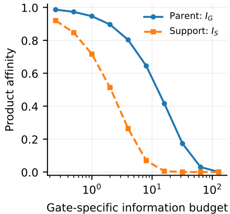
(a) Test-side gates
