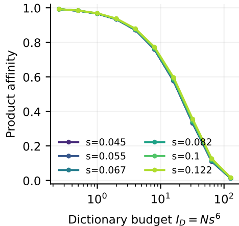
(c) Dictionary-gate collapse
