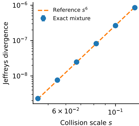
(b) Cubic-score geometry
