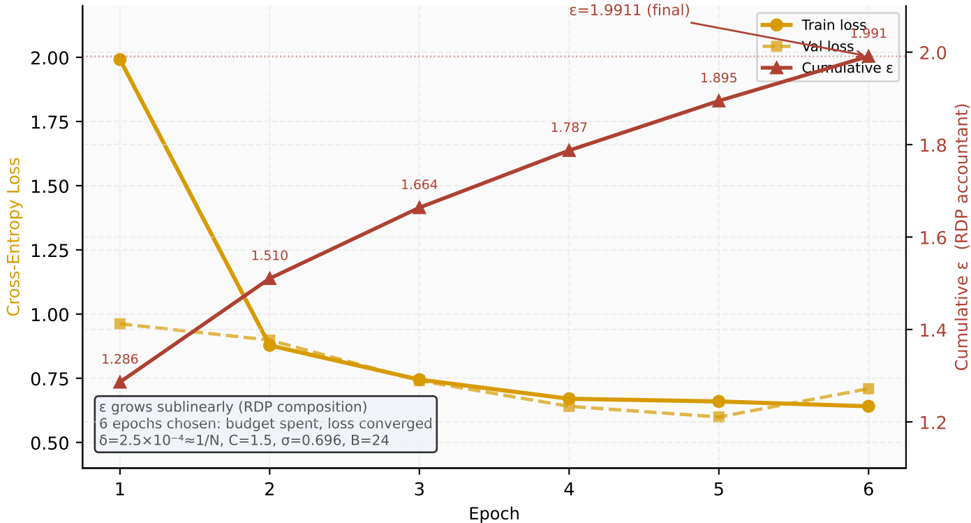
F: DP-QLoRA Training Dynamics ( \epsilon \approx 2 ) RDP accountant tracks \epsilon epoch-by-epoch
