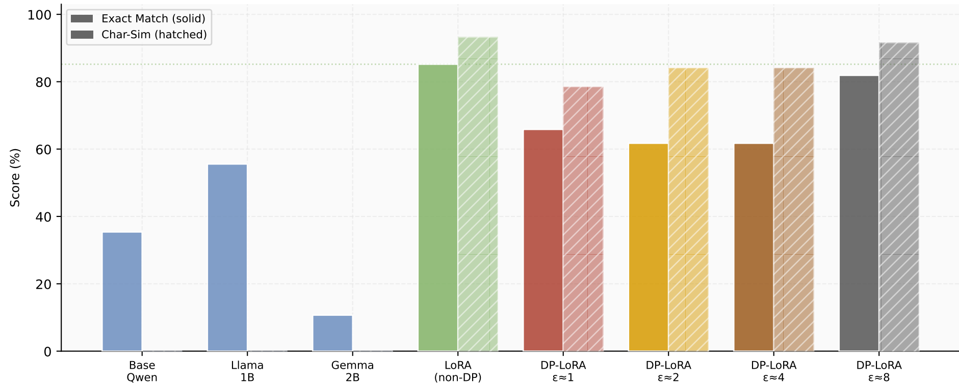
G: Full Model Comparison EM (solid) vs Char-Sim (hatched)
