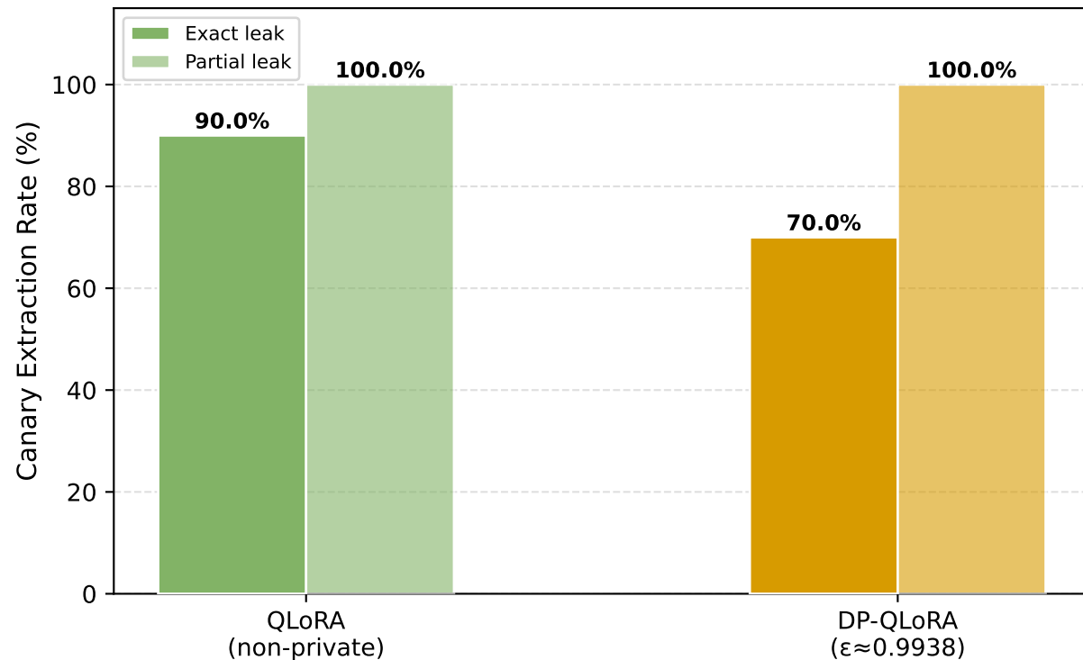
Canary Extraction Attack Lower = stronger privacy
