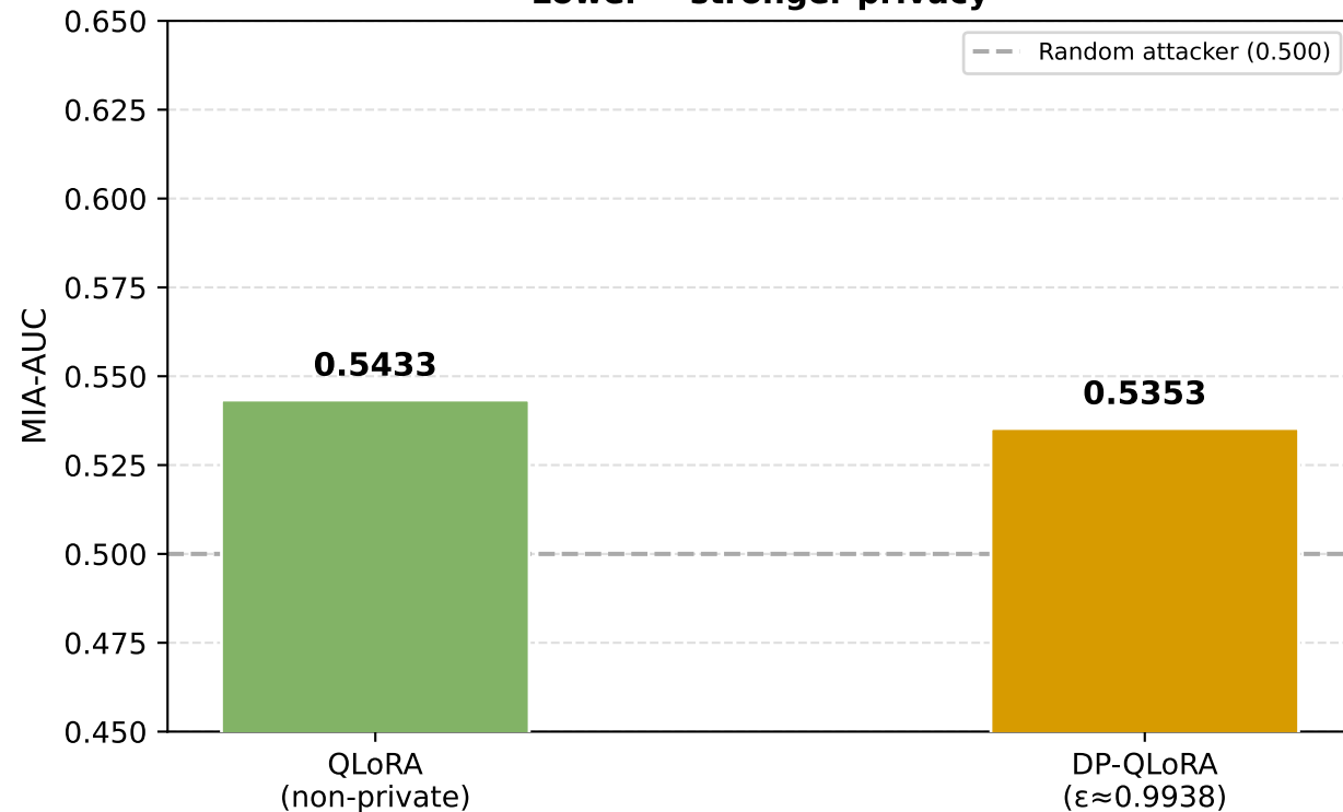
Membership Inference Attack Lower = stronger privacy
