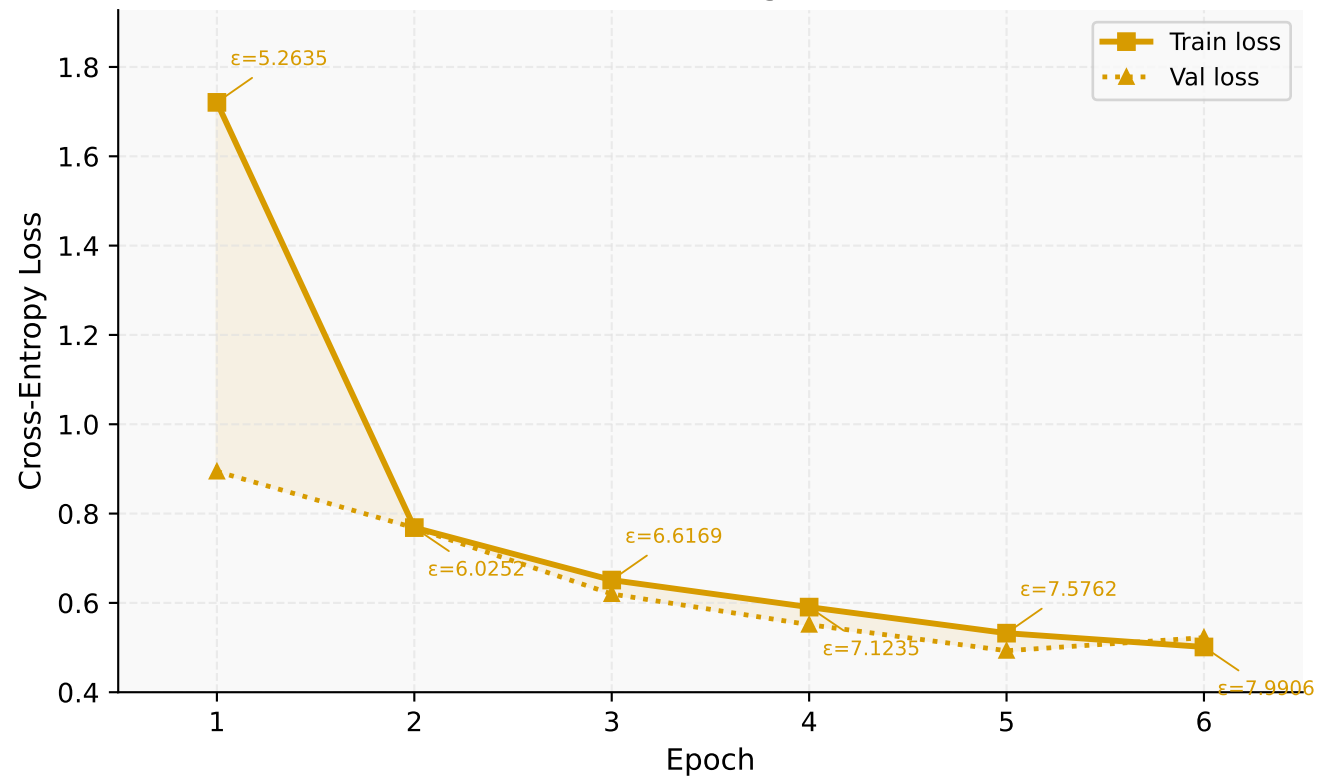
DP-QLoRA ( \epsilon \approx 7.9906 ) Loss Convergence
