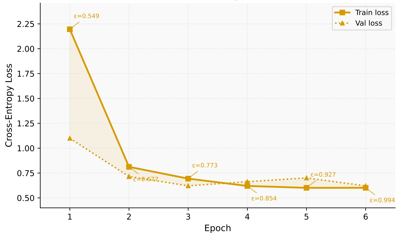
DP-QLoRA ( \epsilon \approx 0.99 ) Loss Convergence
