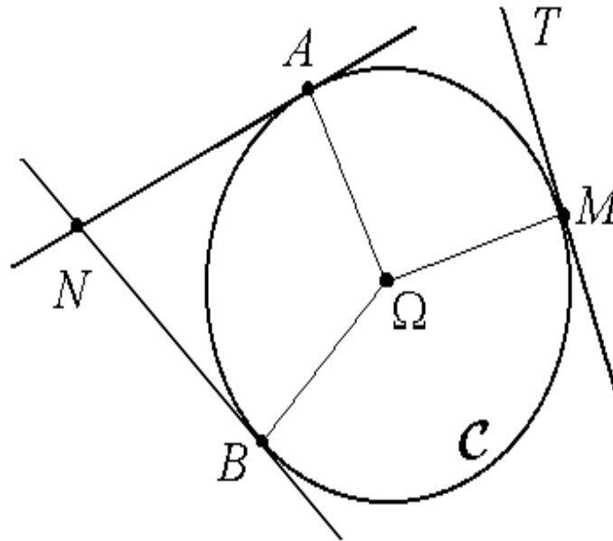
FIGURE 5.4 – Tangentes de cercles
