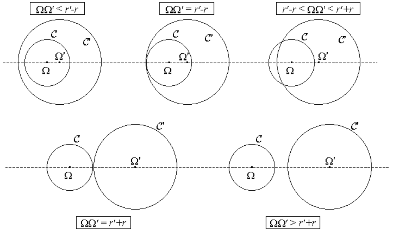
FIGURE 5.5 – Intersection de cercles
