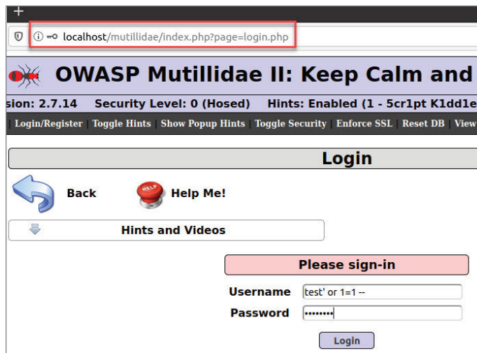
Figure 8.16: Mutillidae – Login SQLi
