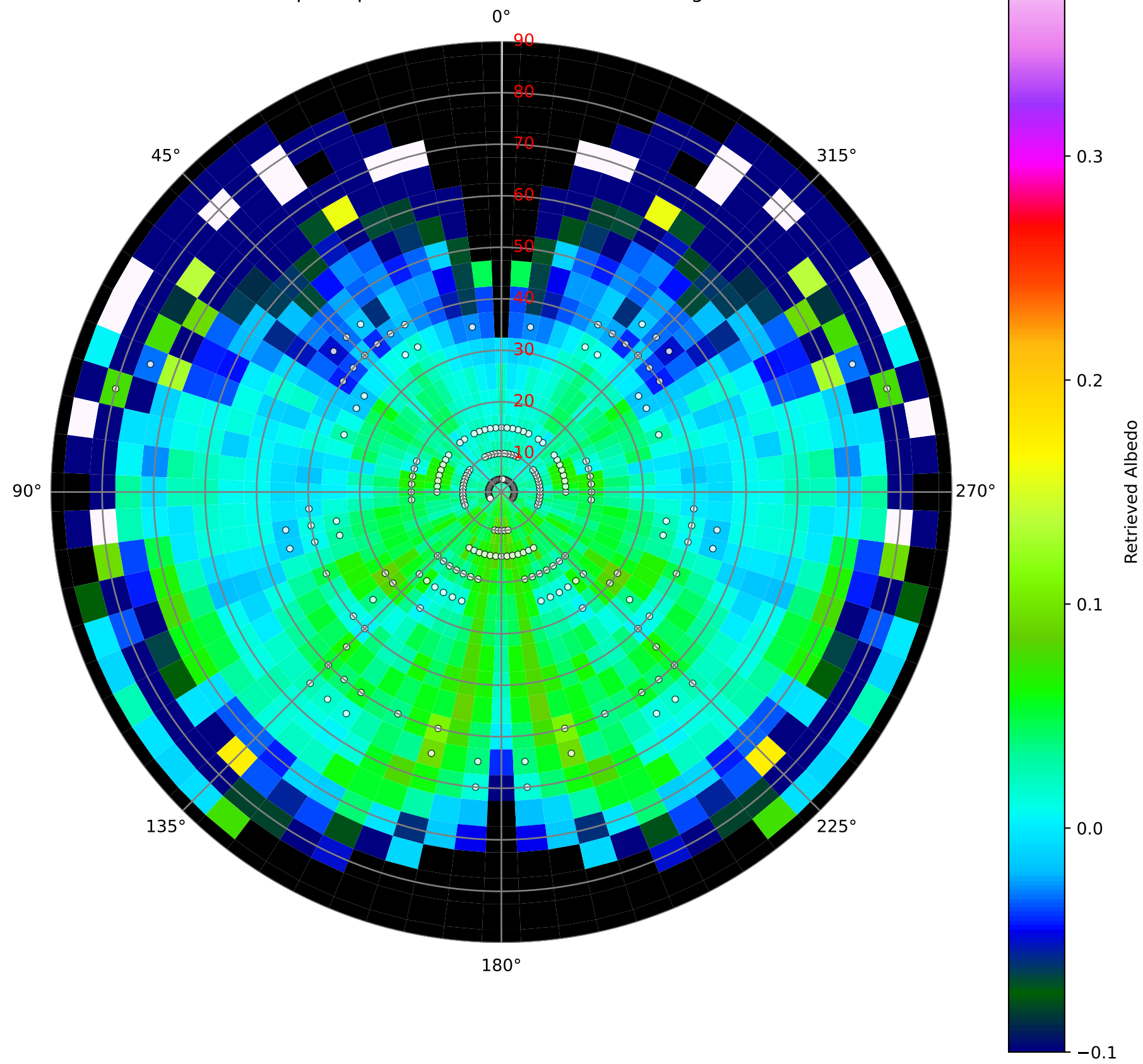
1.27 \mu m Equatorial Dunes. Incidence: 55 degrees
