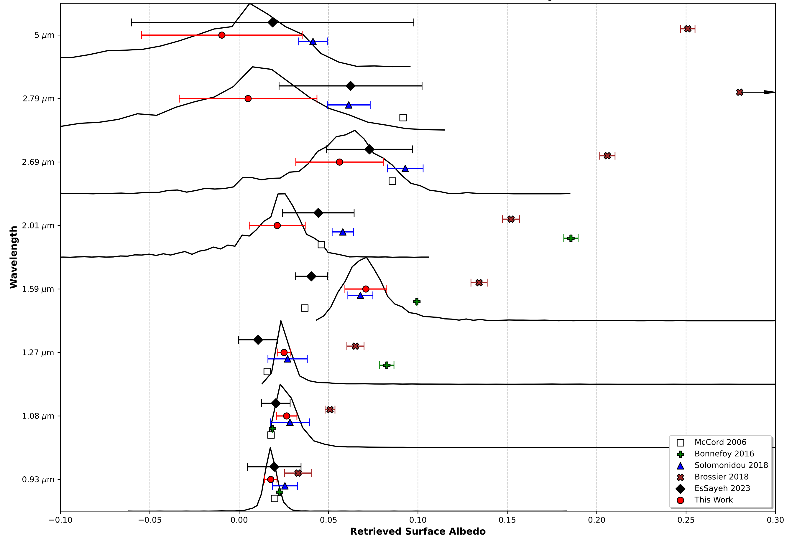
Distribution of Retrieved Albedos -- Emission \leq 40 degrees#
