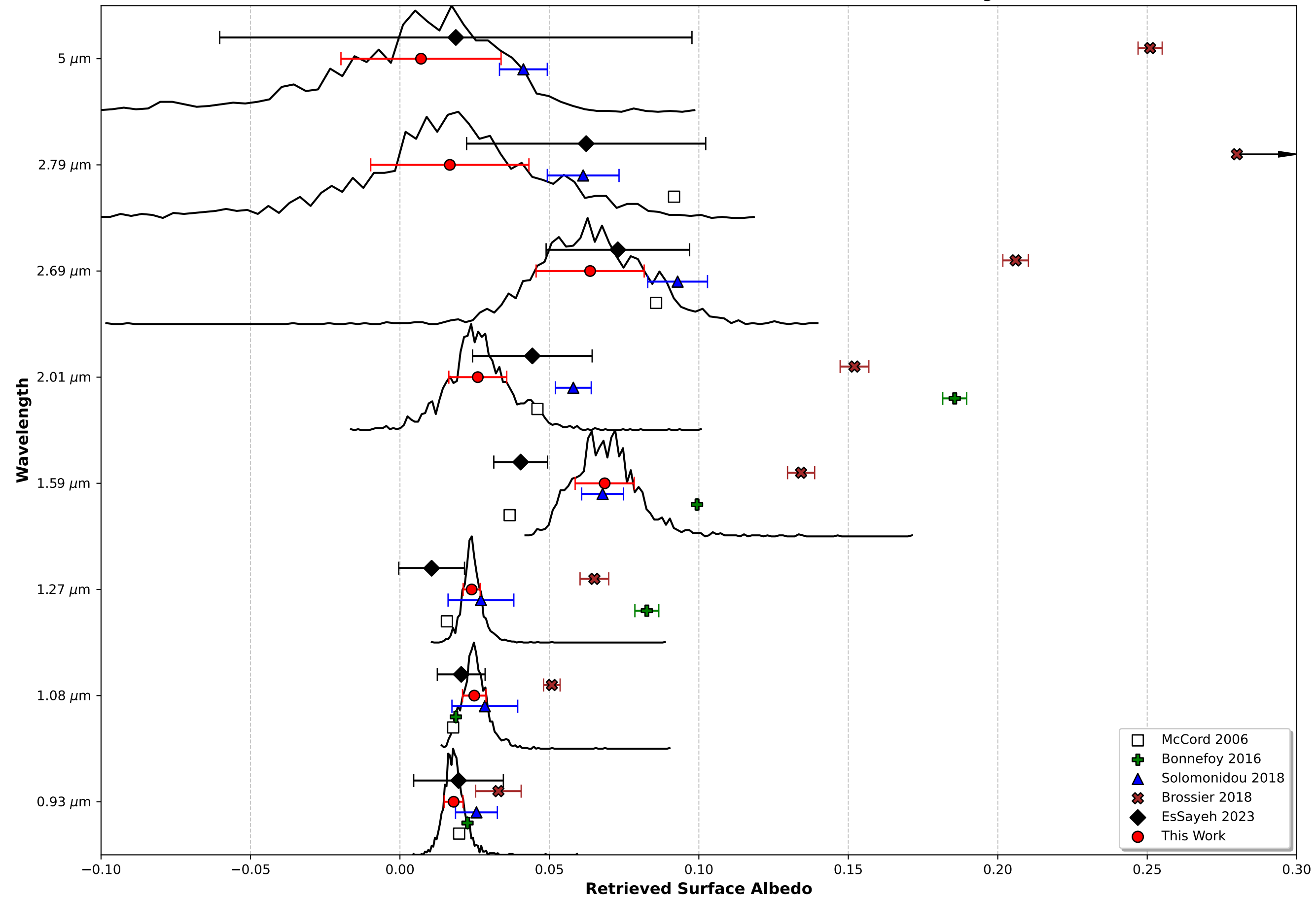
Distribution of Retrieved Albedos -- Incidence and Emission \leq 40 degrees#
