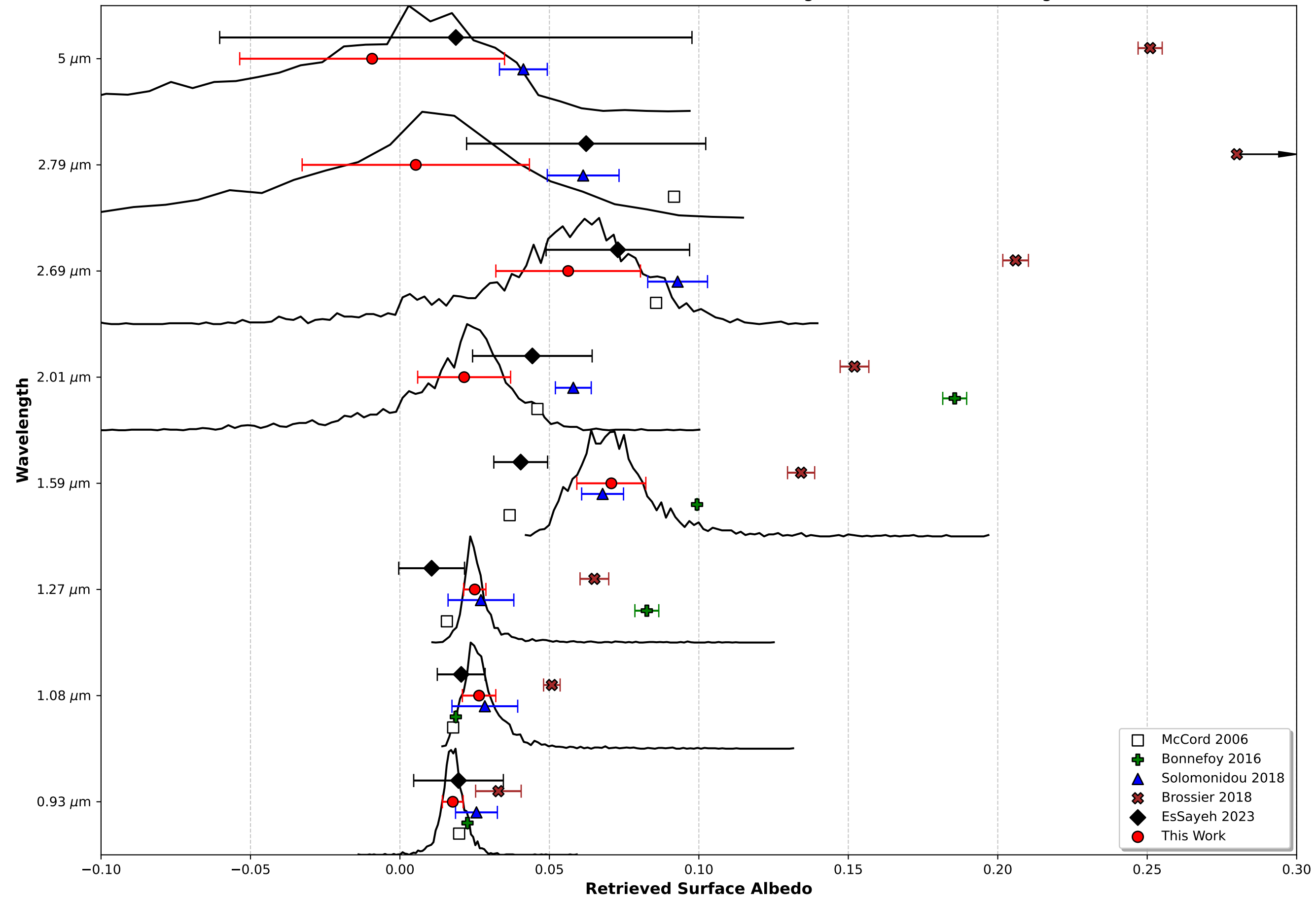
Distribution of Retrieved Albedos -- Emission \leq 40 degrees, Incidence \leq 80 degrees
