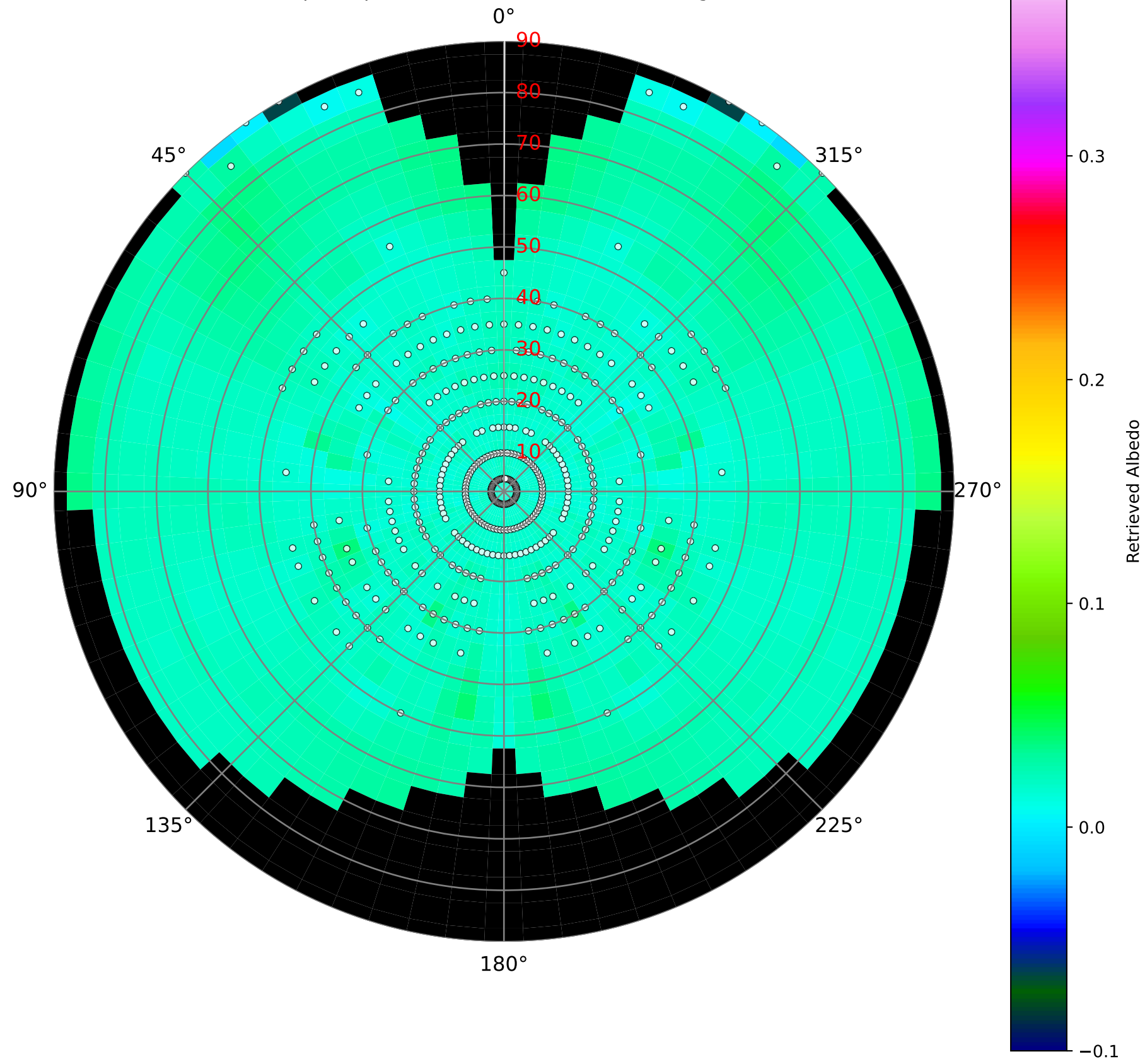
5.00 \mu\text{m} Equatorial Dunes. Incidence: 35 degrees
