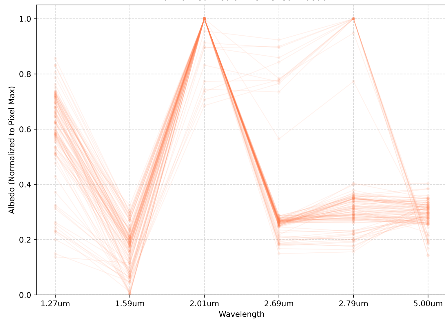
Normalized Median Retrieved Albedo
