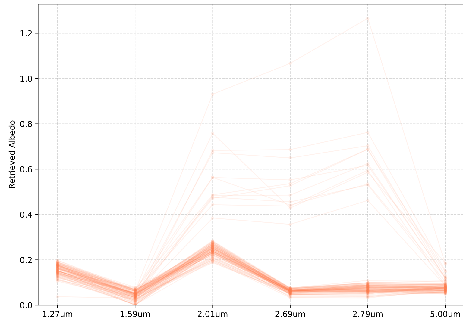
Normalized Median Retrieved Albedo
