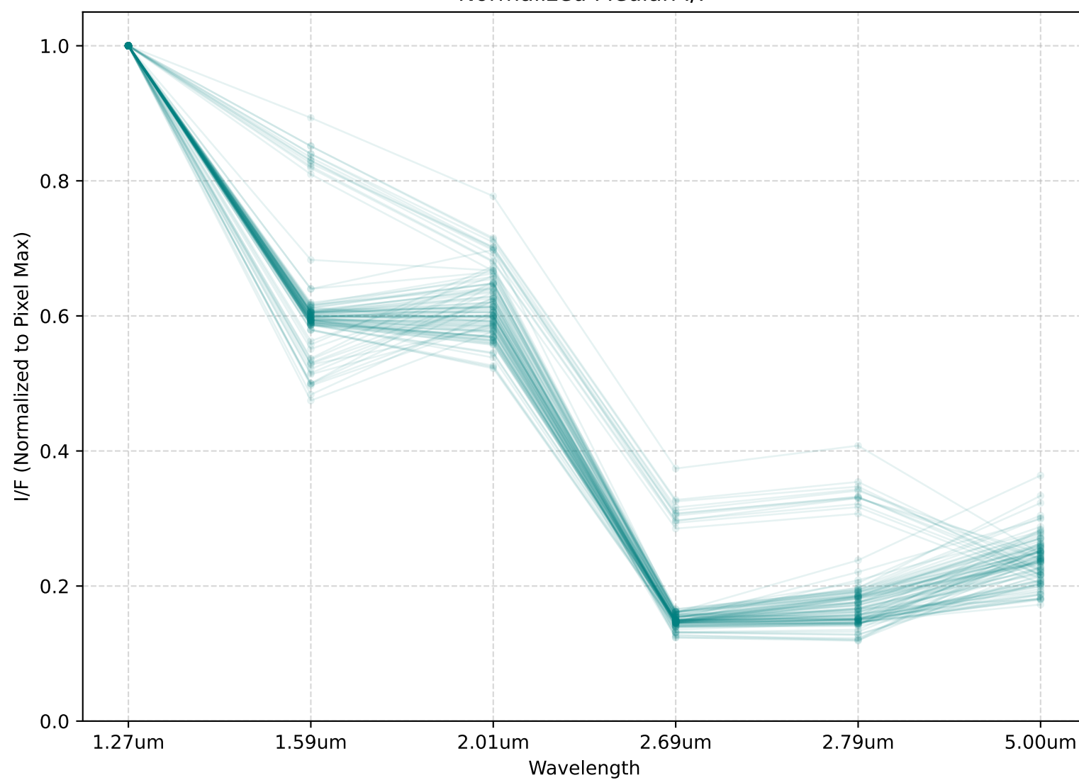
Normalized Median I/F
