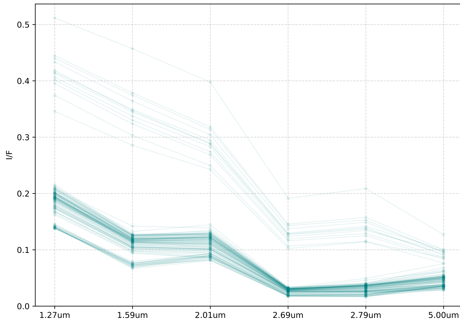
Normalized Median I/F
