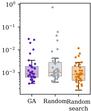
Heat conduction
