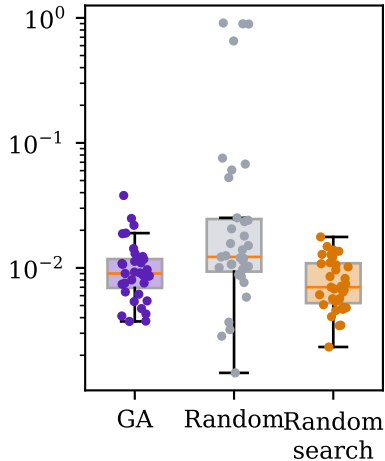
Vibrating string
