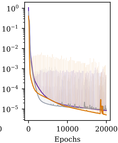
Heat conduction (run 32)
