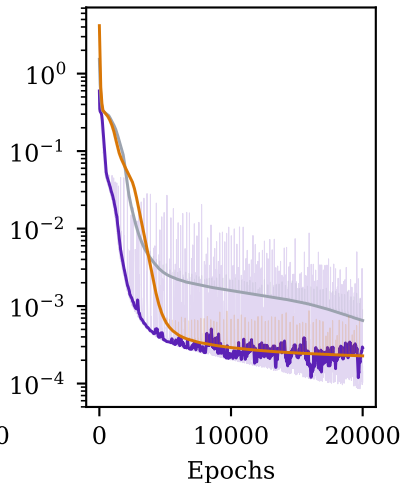
Vibrating string (run 0)
