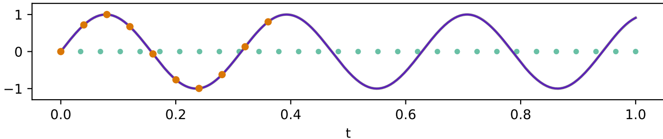
PINN (data + physics loss, 20,000 epochs) — L^2 = 0.003
