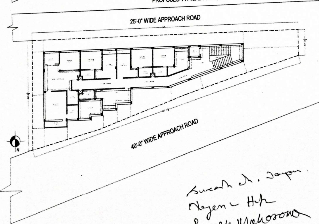
PROPOSED TYPICAL FIRST, SECOND, THIRD & FOURTH FLOOR PLAN
