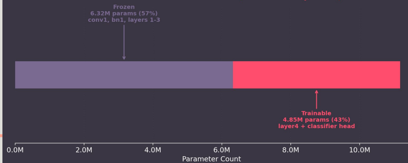
ResNet-18 Parameter Breakdown (11.18M total params)
