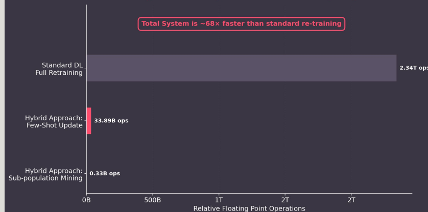
Operational Multiplier: Scientific Time Complexity
