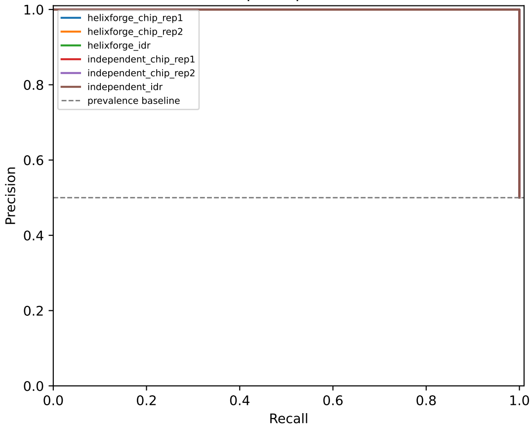
Candidate-panel precision-recall
