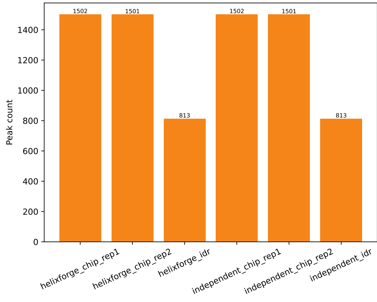
Replicate and IDR peak-set sizes
