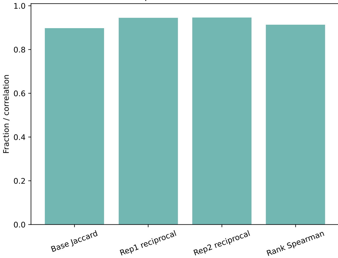
Replicate concordance
