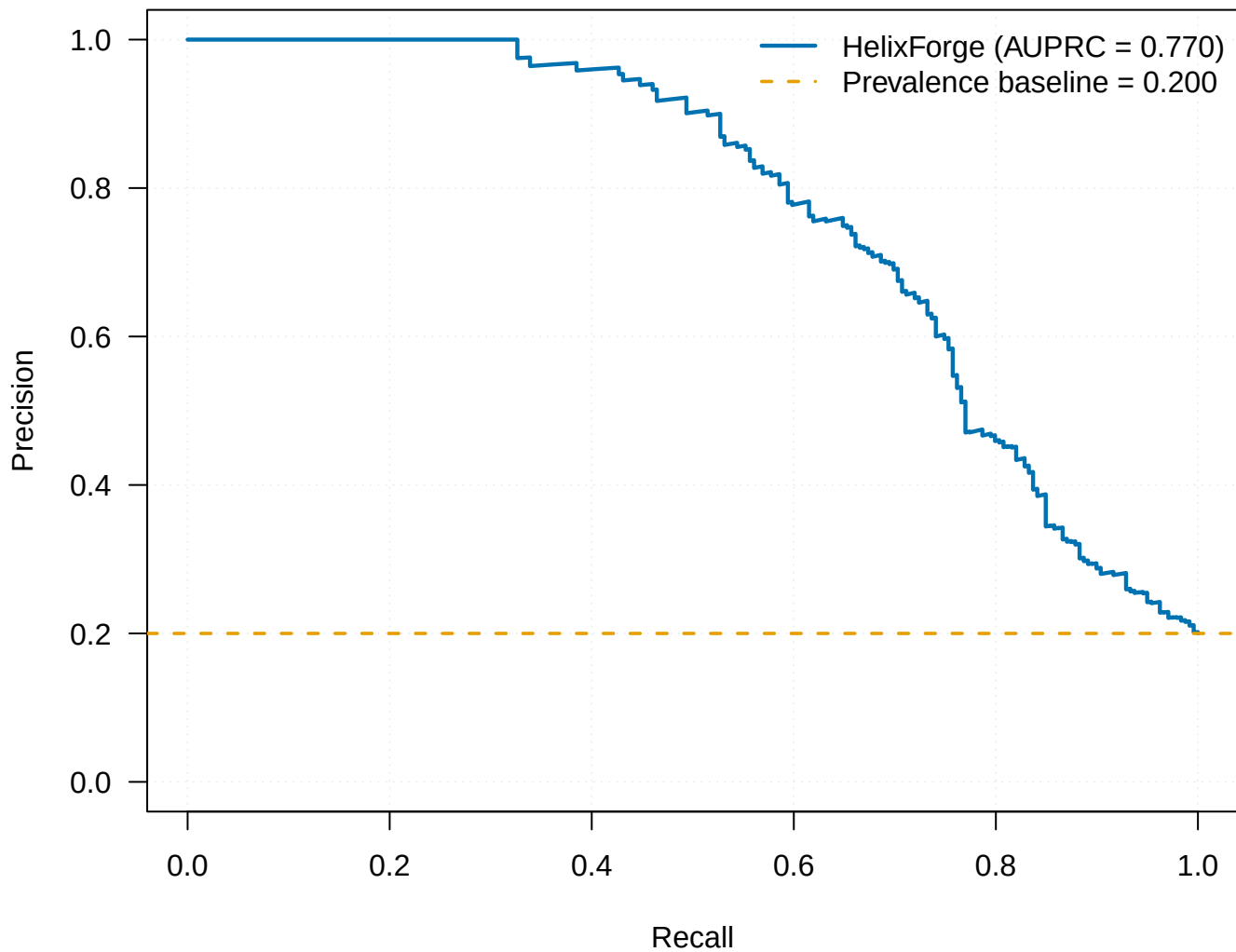
Precision–recall curve for synthetic differential expression
